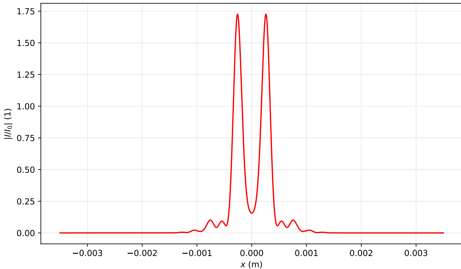
Intensity profile I(x, y = 0, z = 0.955)/I_0 , P_{in}=3.5P_{cr} , artificial time
